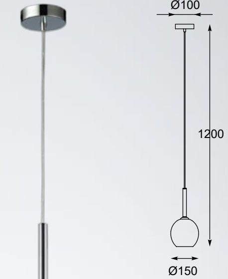
MONIC Pendant lamp MD1629-1 Chrome 1xE14 MAX 40W smoky chrome glass with chrome canopy
